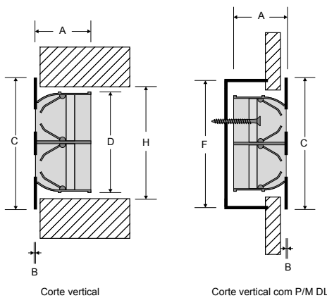
Corte vertical
